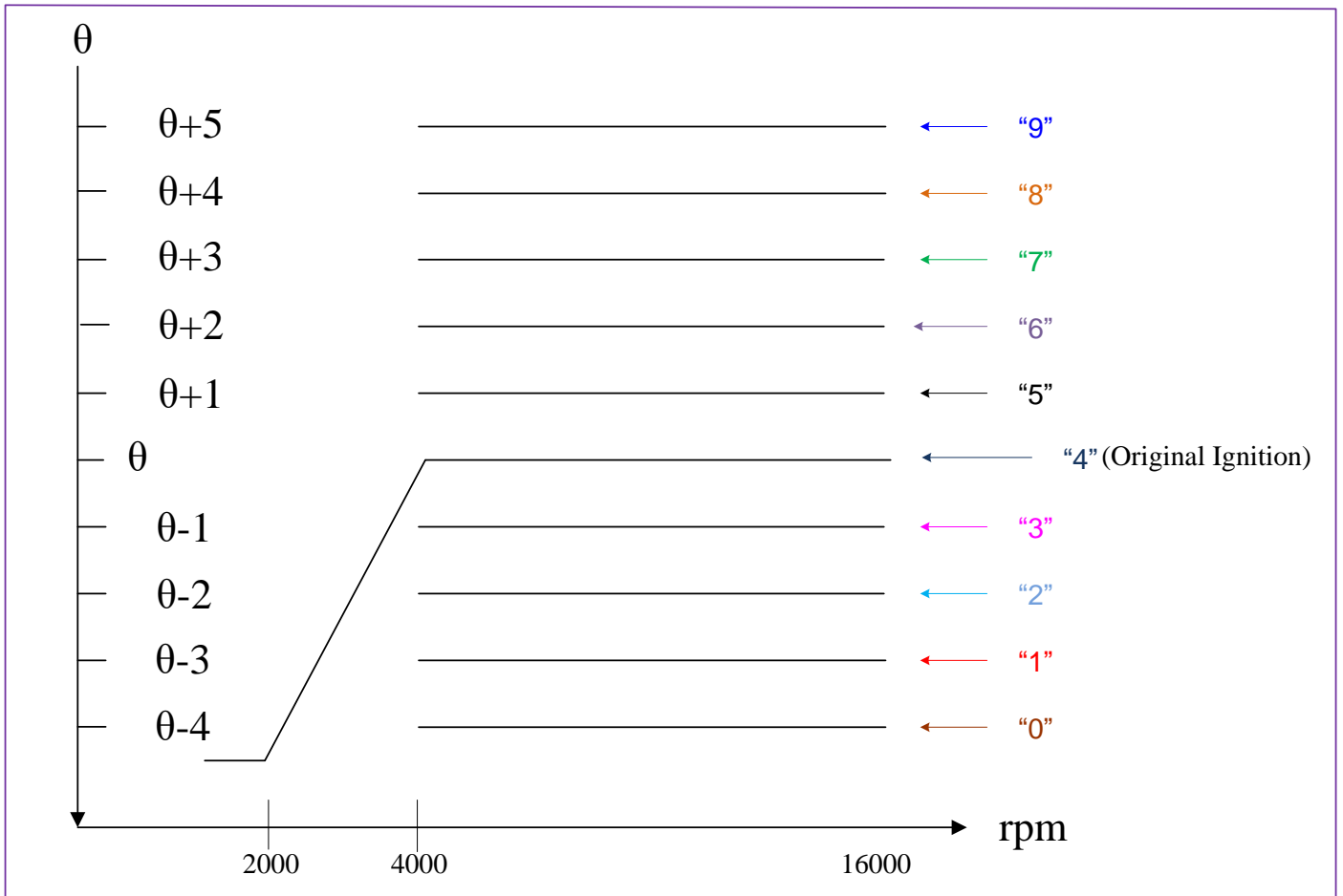
Ignition timing
