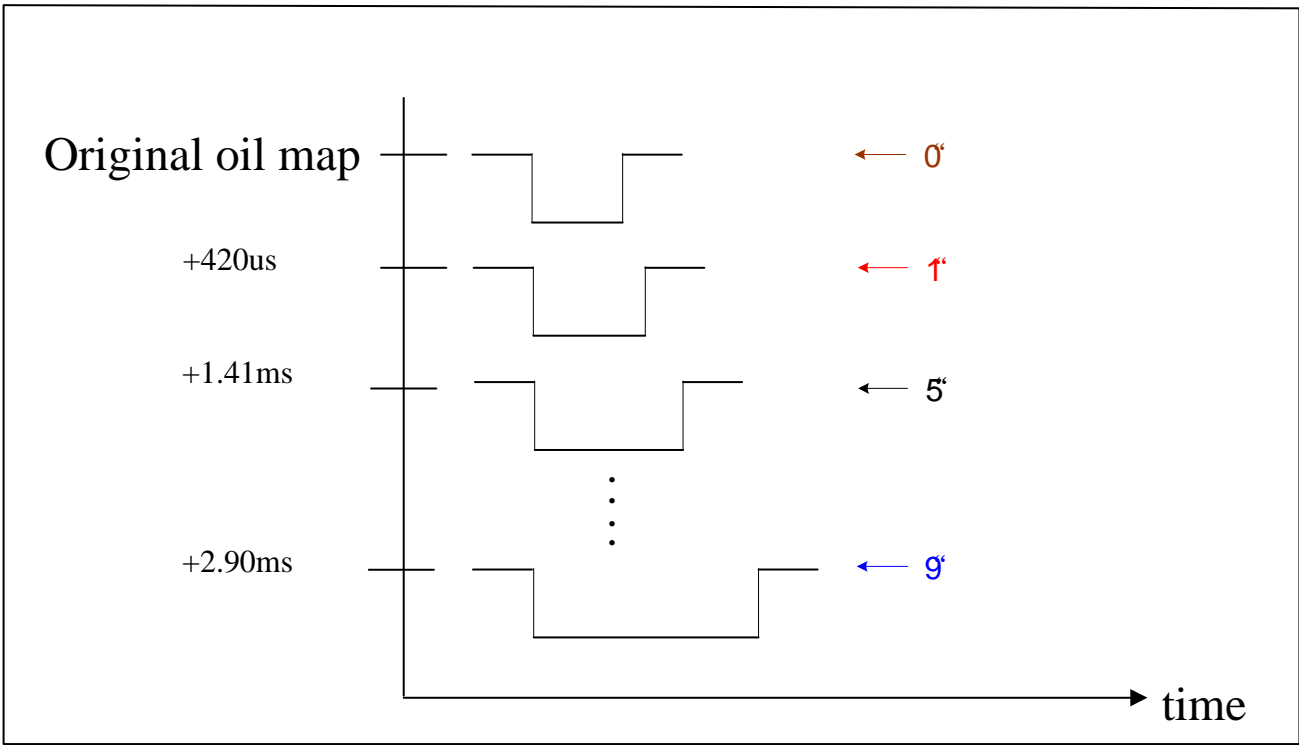
Oil timing
